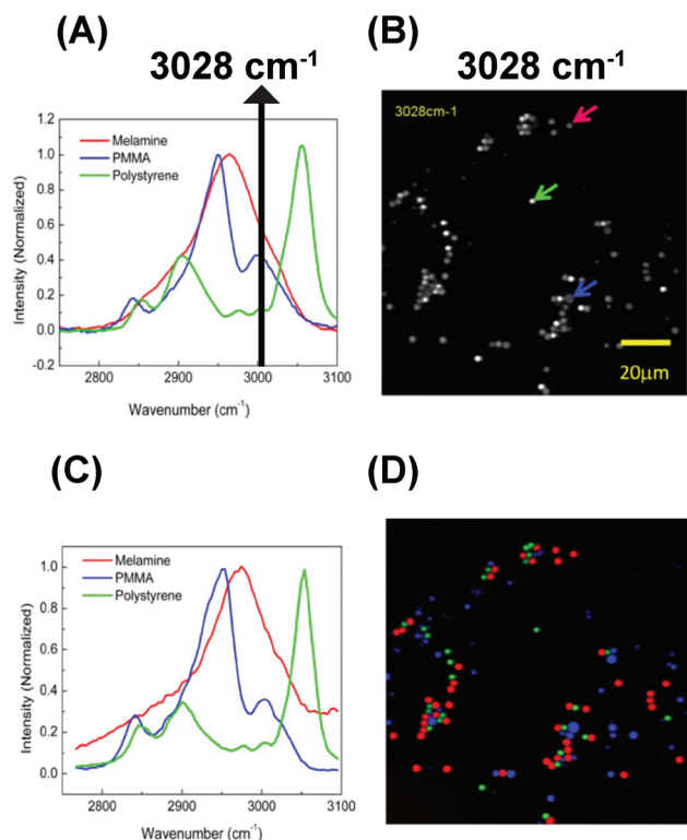
Fig. 5 Hyperspectral stimulated Raman scattering (hSRS) imaging for mapping three types of polymer beads with overlapping but distinct Raman spectra (A) spontaneous Raman spectra of the three polymer beads. The black solid line indicates overlapping Raman spectra at 3028\text{ cm}^{-1} (B) stimulated Raman scattering (SRS) imaging of the three polymer beads at 3028\text{ cm}^{-1} with different color arrows pointing out corresponding beads (C) SRS spectra for the three polymer beads pointed out by the arrows (in B). (D) Color-code distribution of the three polymer beads generated using hSRS imaging coupled with spectral decomposition. PMMA: poly (methyl methacrylate). Reprinted with permission from ref. 87 Copyright (2018) American Chemical Society.
