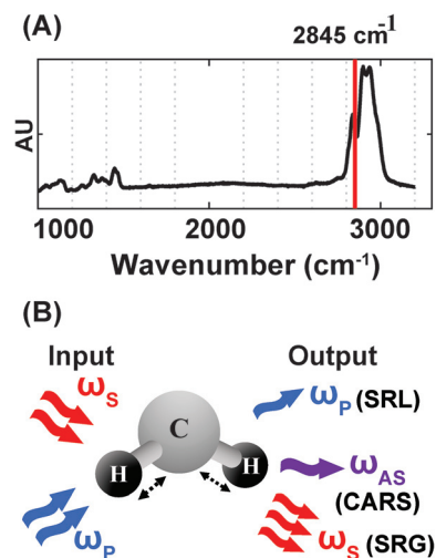
Fig. 2 Vibrational imaging of lipids using coherent Raman scattering. (A) Spontaneous Raman spectra of oleic acid. The red solid line indicates asymmetric stretching vibrational mode of the carbon–hydrogen bond at 2845 cm −1 . (B) Schematic of excitation and detection for coherent Raman scattering. For both coherent anti-stokes Raman scattering (CARS) and stimulated Raman scattering (SRS) imaging, a characteristic vibrational mode of the CH 2 bond in lipids is excited with two incoming photons at the pump ( \omega_p ) and Stokes ( \omega_s ) frequency. Stimulated Raman loss (SRL) is detected as a loss in the pump intensity and stimulated Raman gain (SRG) is detected as a gain in the Stokes intensity. CARS is detected at the anti-stokes frequency, \omega_{AS} .
